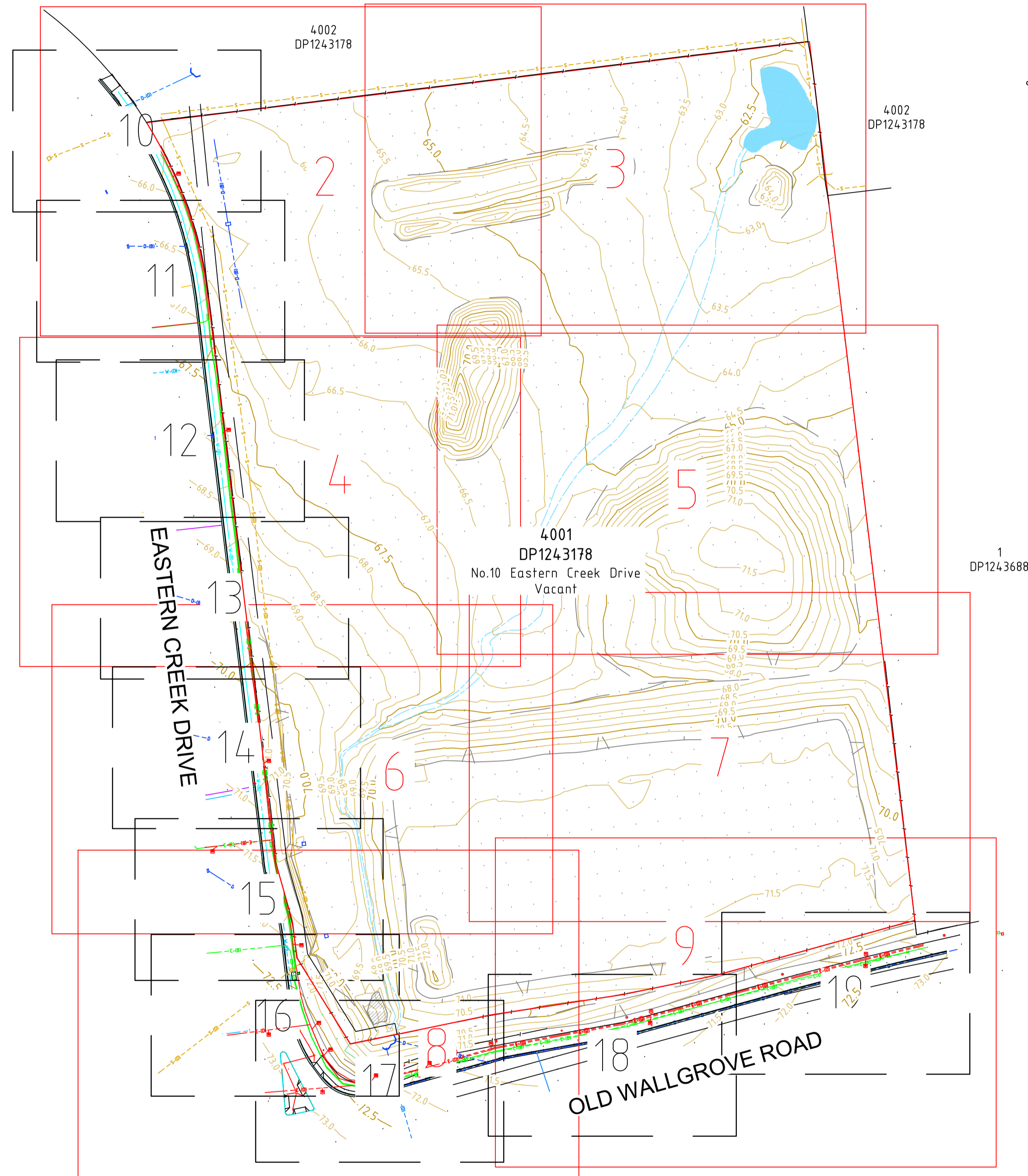
LOCALITY PLAN (Scale 1:1000)
